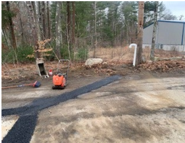
Photo 3: Installation of 4" PVC Manhole Air Vent near Utility Pole #90
